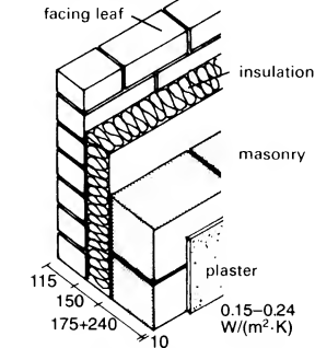
⑥ Aerated concrete cavity wall 0.15-0.24 W/(m 2 ·K)
